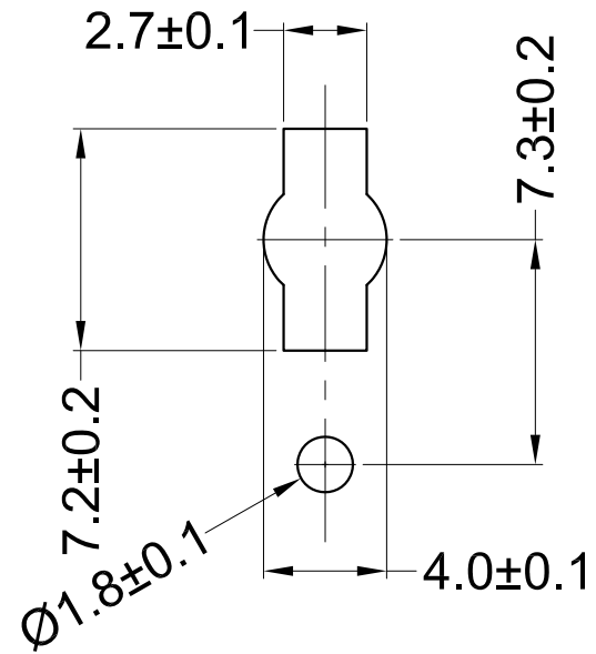
Mounting Hole Detail Panel Thickness:0.8-1.6mm.
