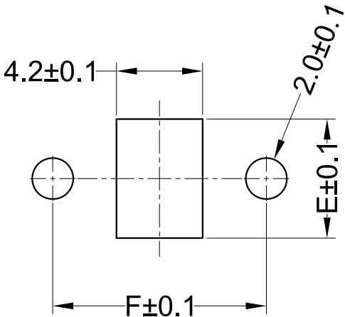
Mounting Hole Detail
