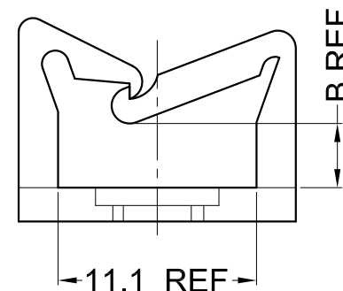
LOCKED POSITION
