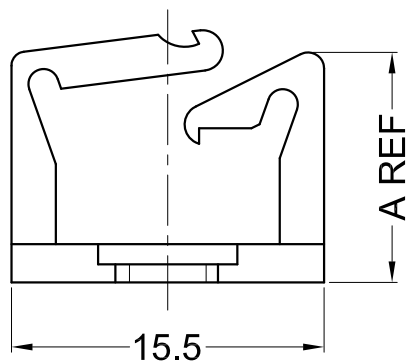
AS MOLDED POSITION
