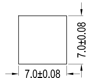
Mounting Hole Panel Thickness: 0.51-3.56mm
