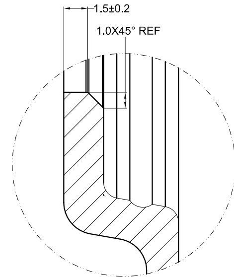
DETAIL B SCALE 5:1
